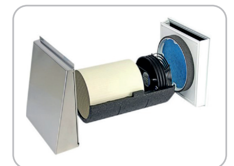
for example: heat recovery unit SEVi 160 Standard
